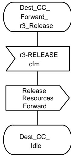
Figure 53 – Stage 2 SDL diagram for Destination CC functional entity (Sheet 9 of 10)
