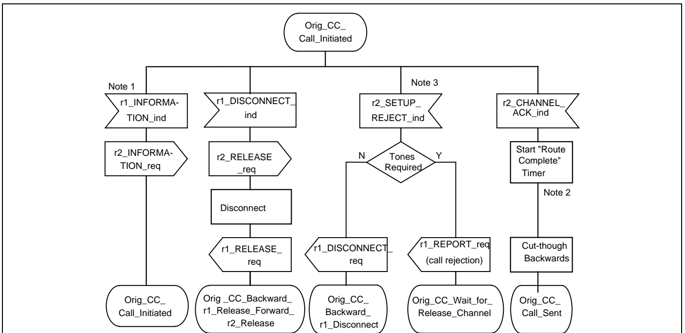
Figure 26 – Stage 2 SDL diagram for Originating CC functional entity (Sheet 2 of 12)
