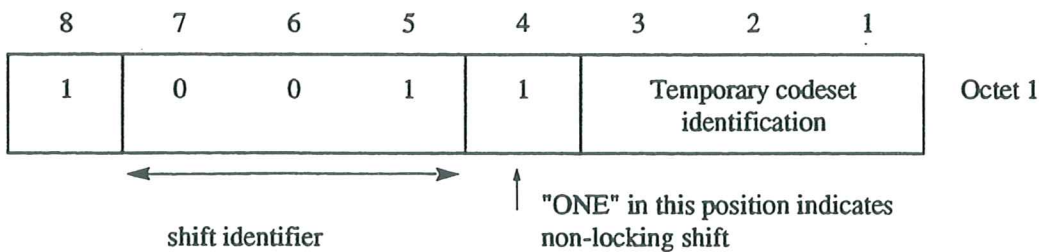
Figure 21 - Non-locking Shift Element
