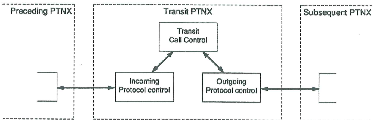
Figure 9 - Relationship of Call control to Protocol Control
