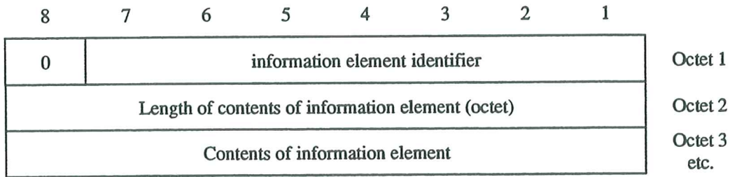
Figure 19 - Variable Length information element Format
