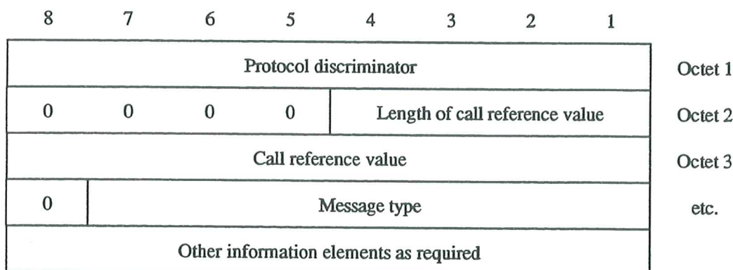
Figure 12 - General Message Organization Example
