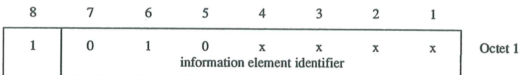
Figure 18 - Single Octet information element Format (type 2)
