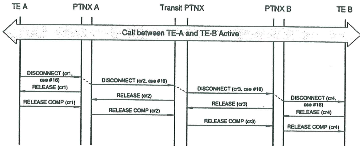
Figure B.5 - Normal Call Clearing by Originator
