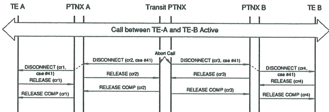
Figure B.6 - Call Abort by Transit PTNX
