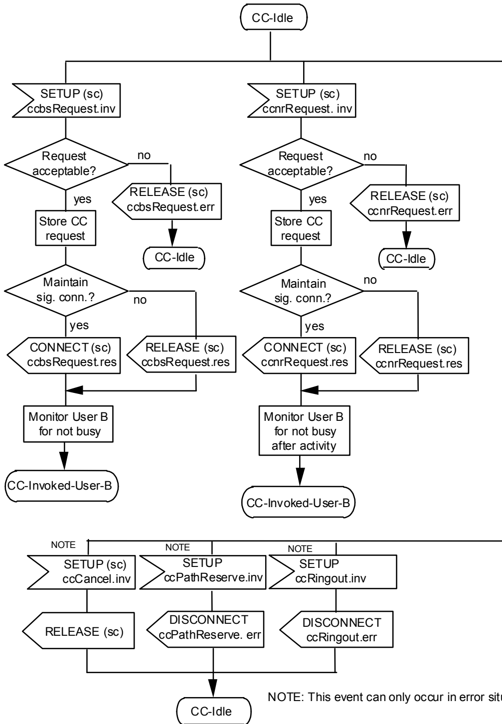
Figure D.11 - Terminating PINX behaviour
