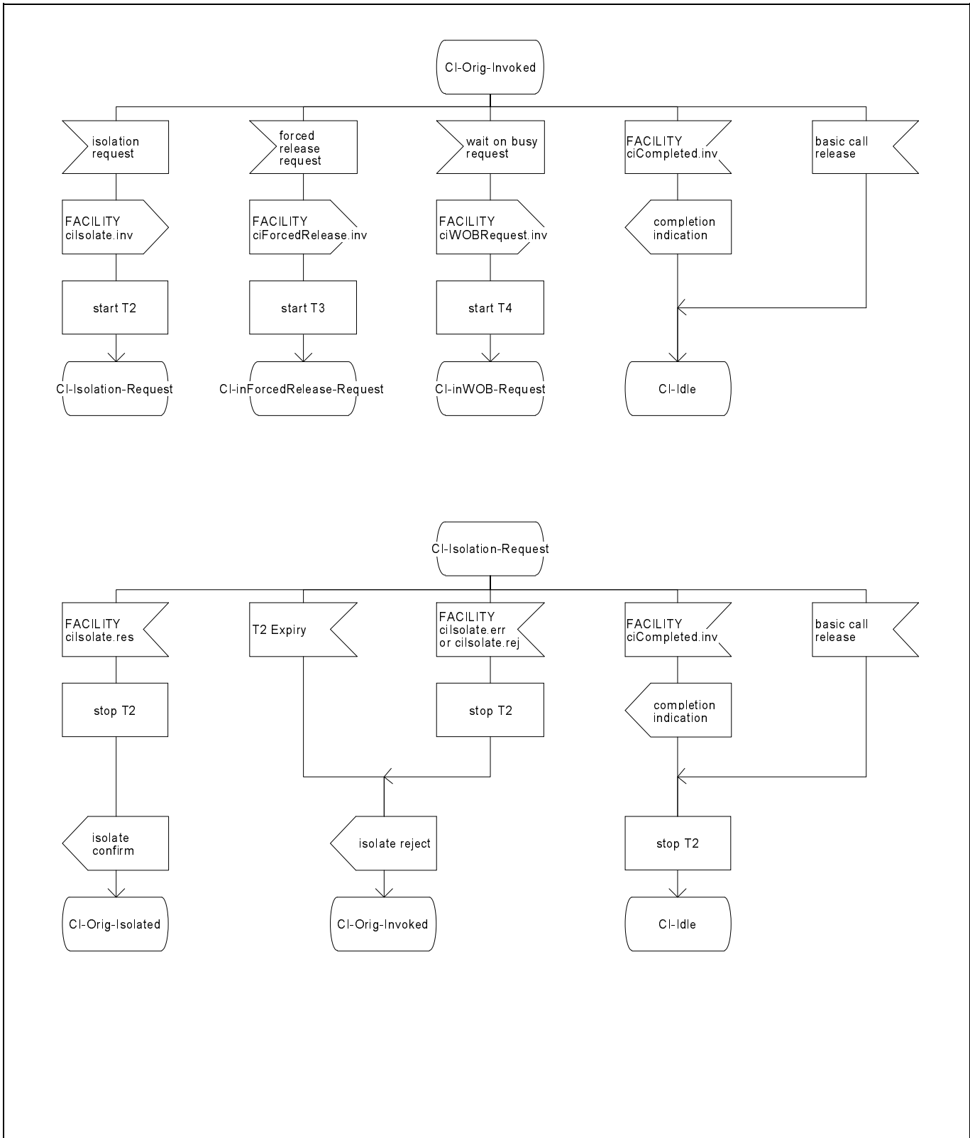
Figure D.1 (sheet 2 of 6) - Originating PTNX SDL
