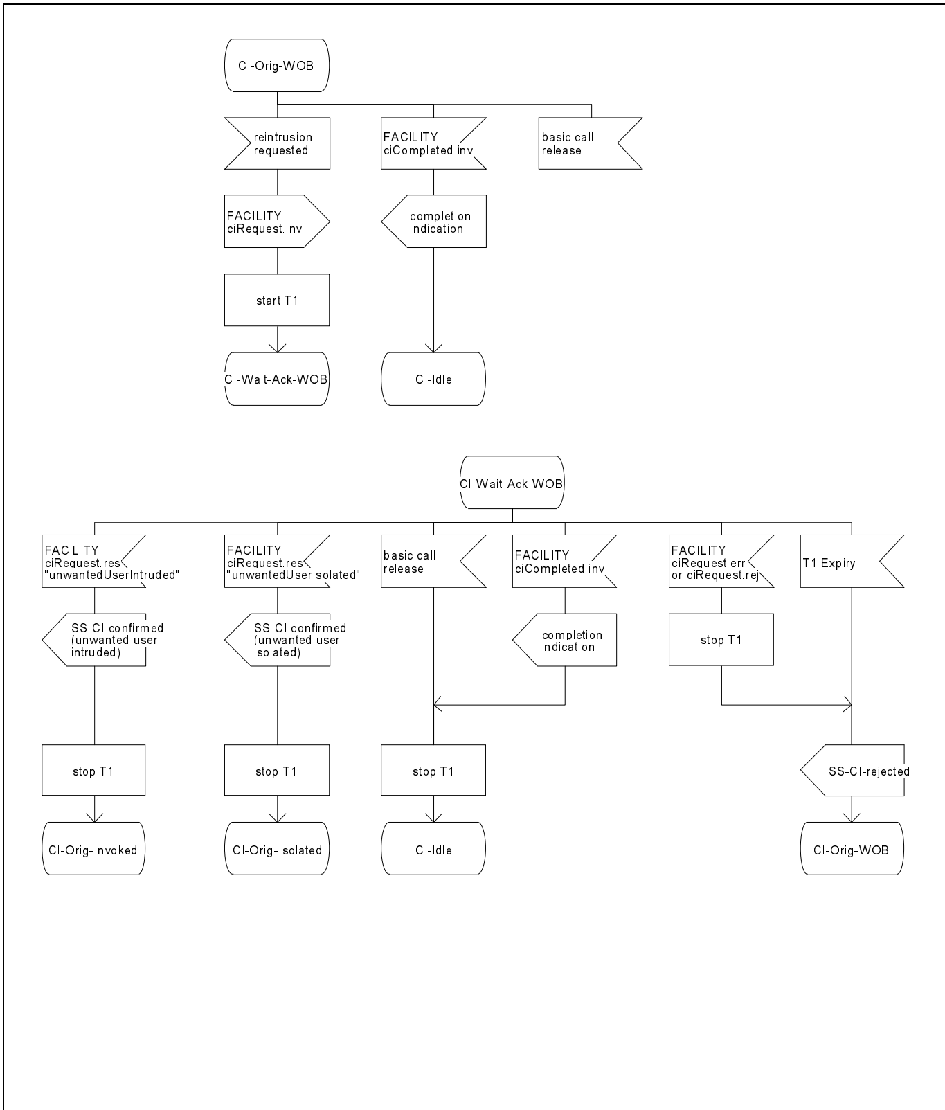
Figure D.1 (sheet 6 of 6) - Originating PTNX SDL
