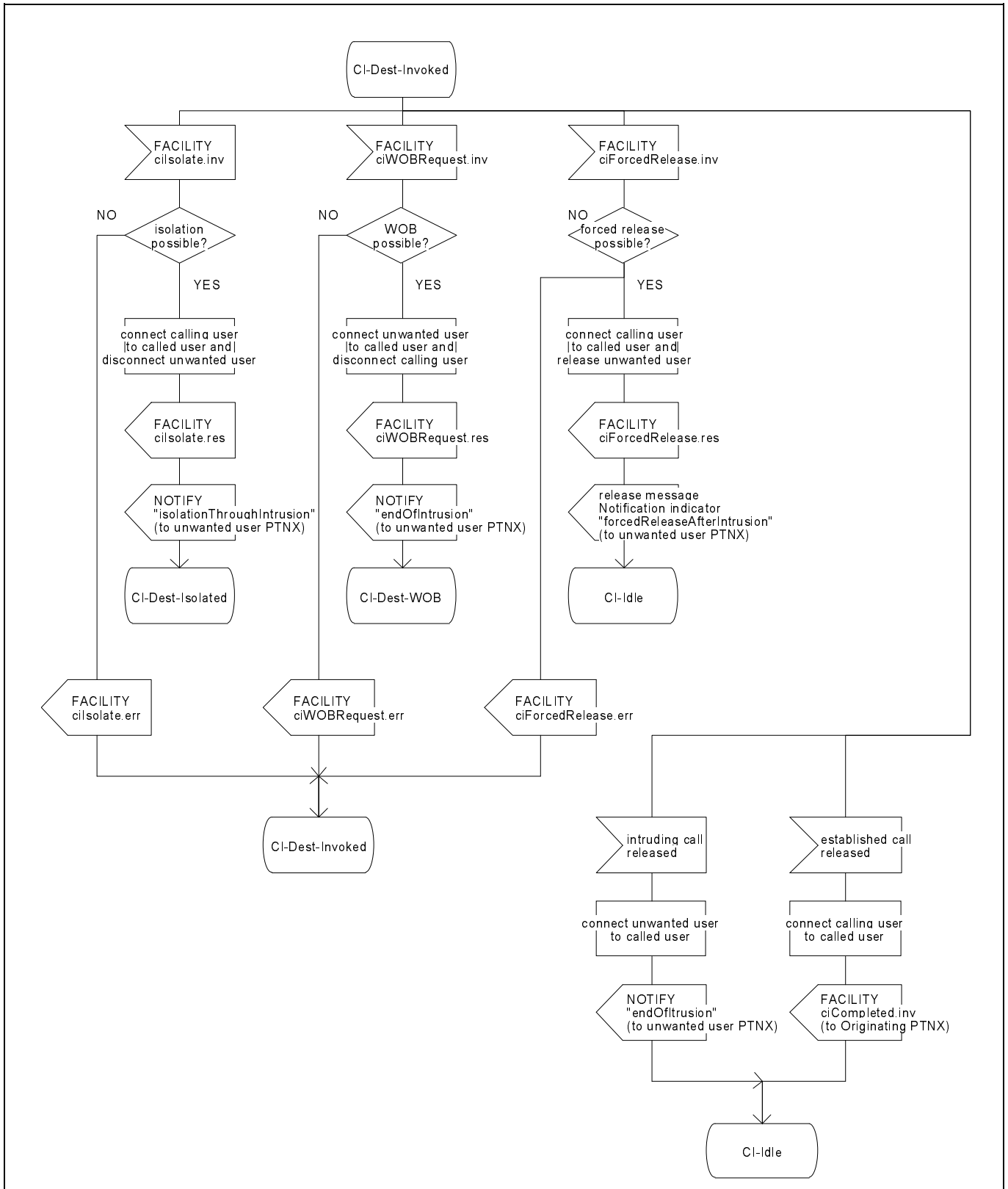
Figure D.2 (sheet 3 of 6) - Terminating PTNX SDL
