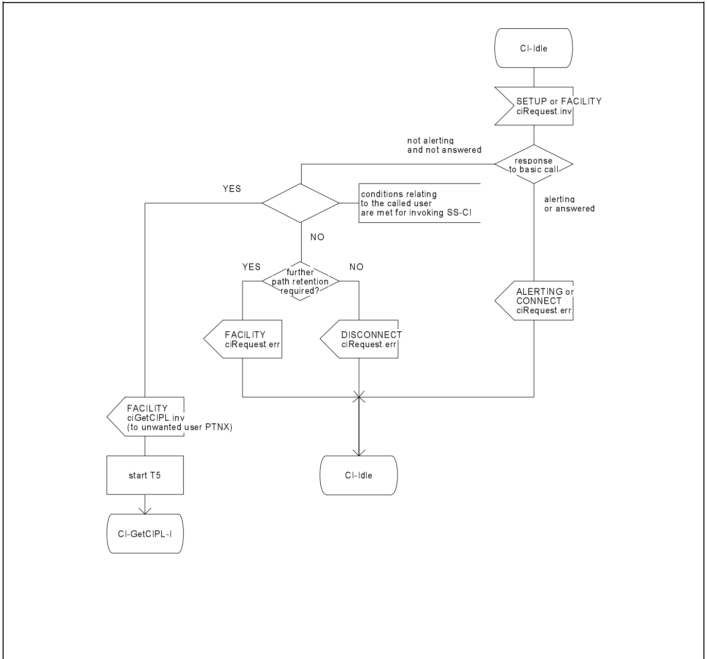
Figure D.2 (sheet 1 of 6) - Terminating PTNX SDL
