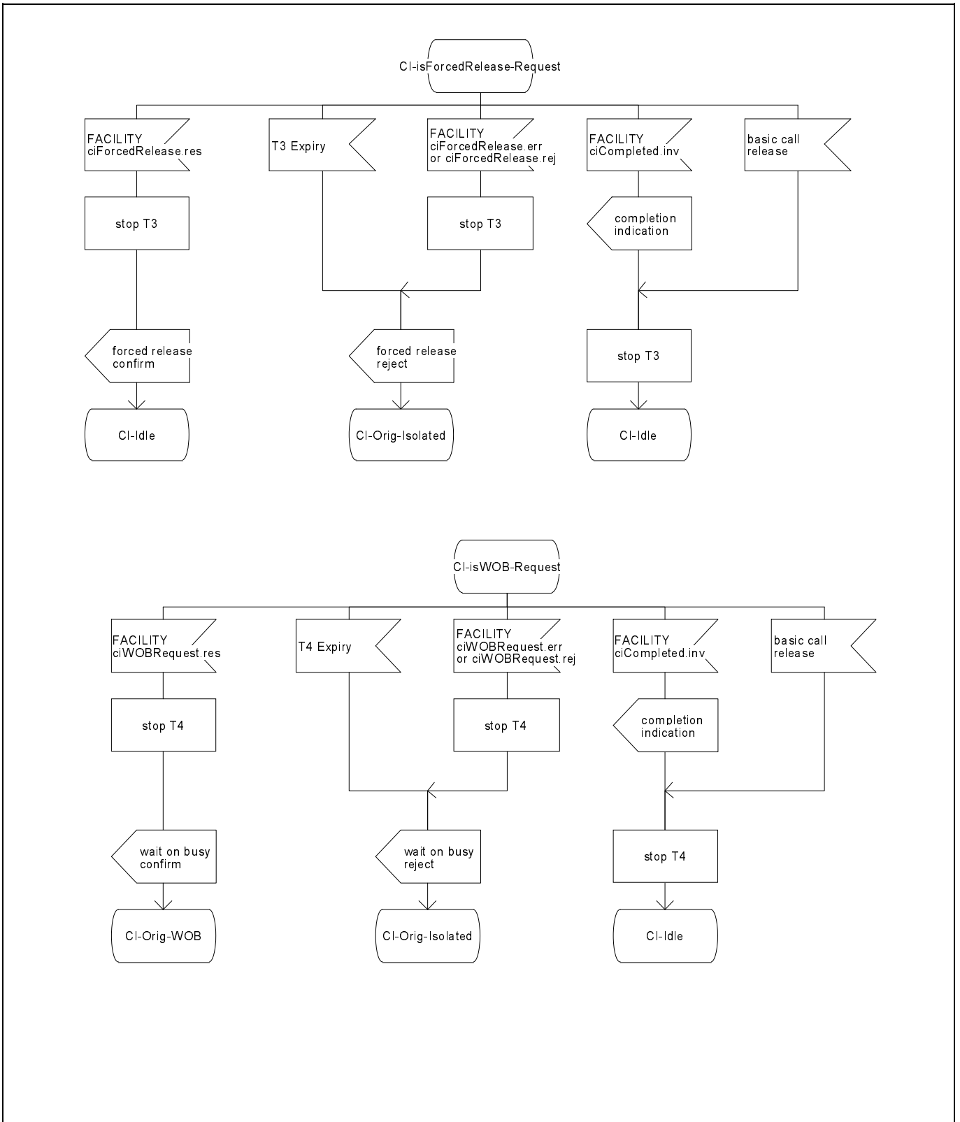
Figure D.1 (sheet 5 of 6) - Originating PTNX SDL
