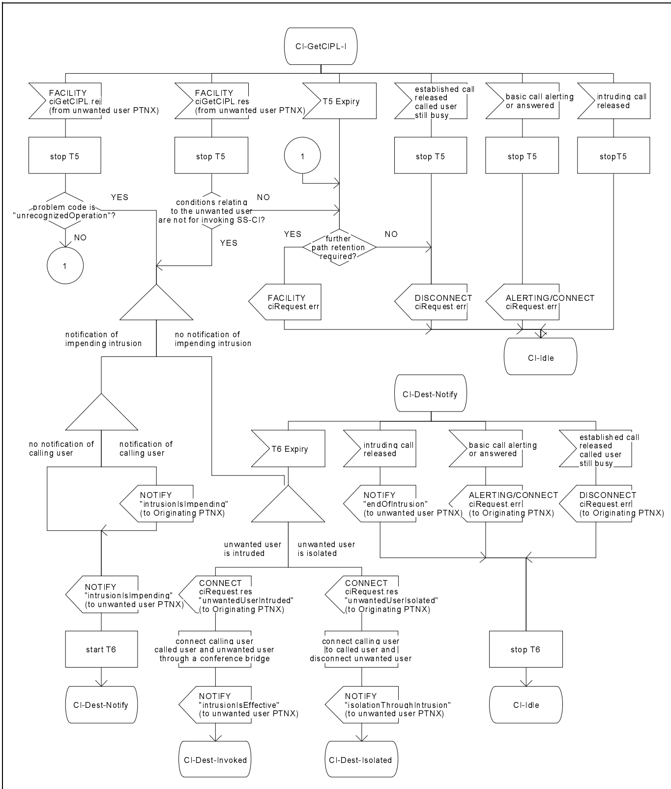
Figure D.2 (sheet 2 of 6) - Terminating PTNX SDL
