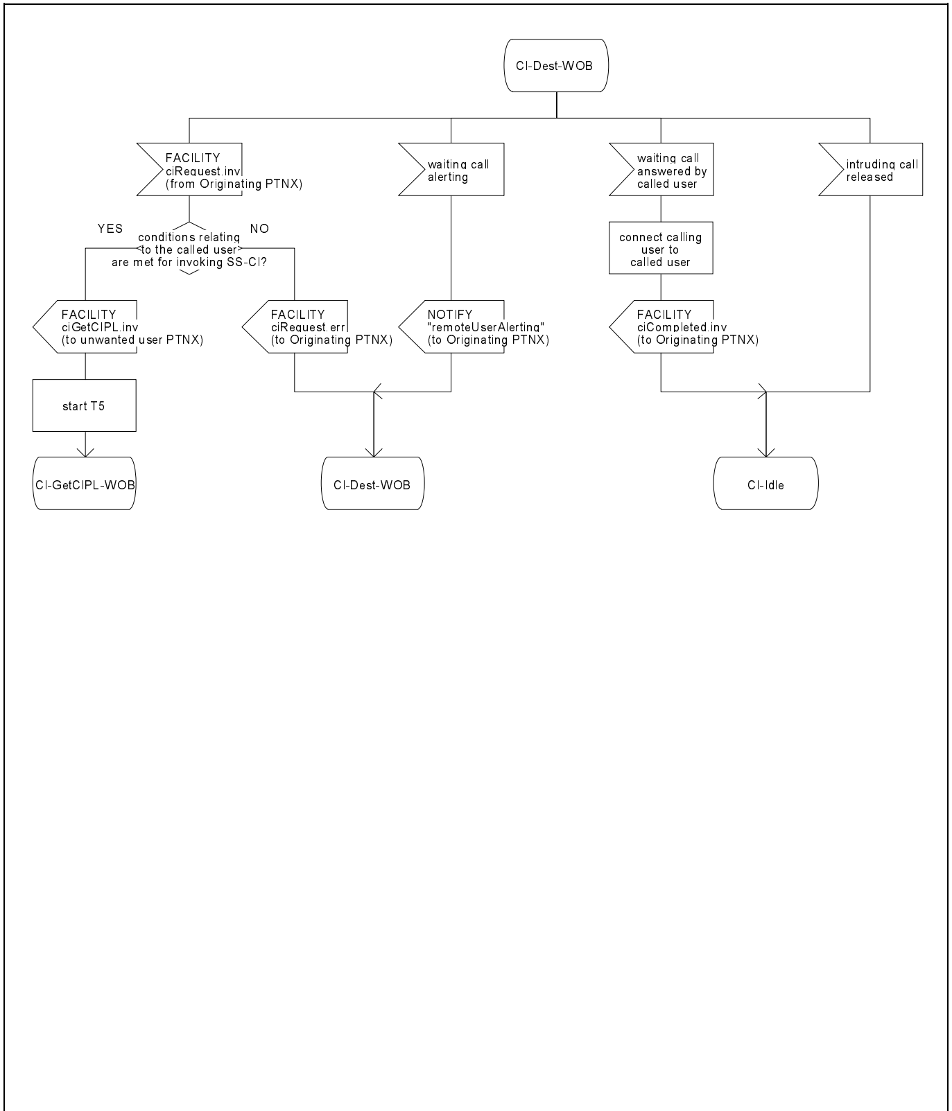
Figure D.2 (sheet 5 of 6) - Terminating PTNX SDL
