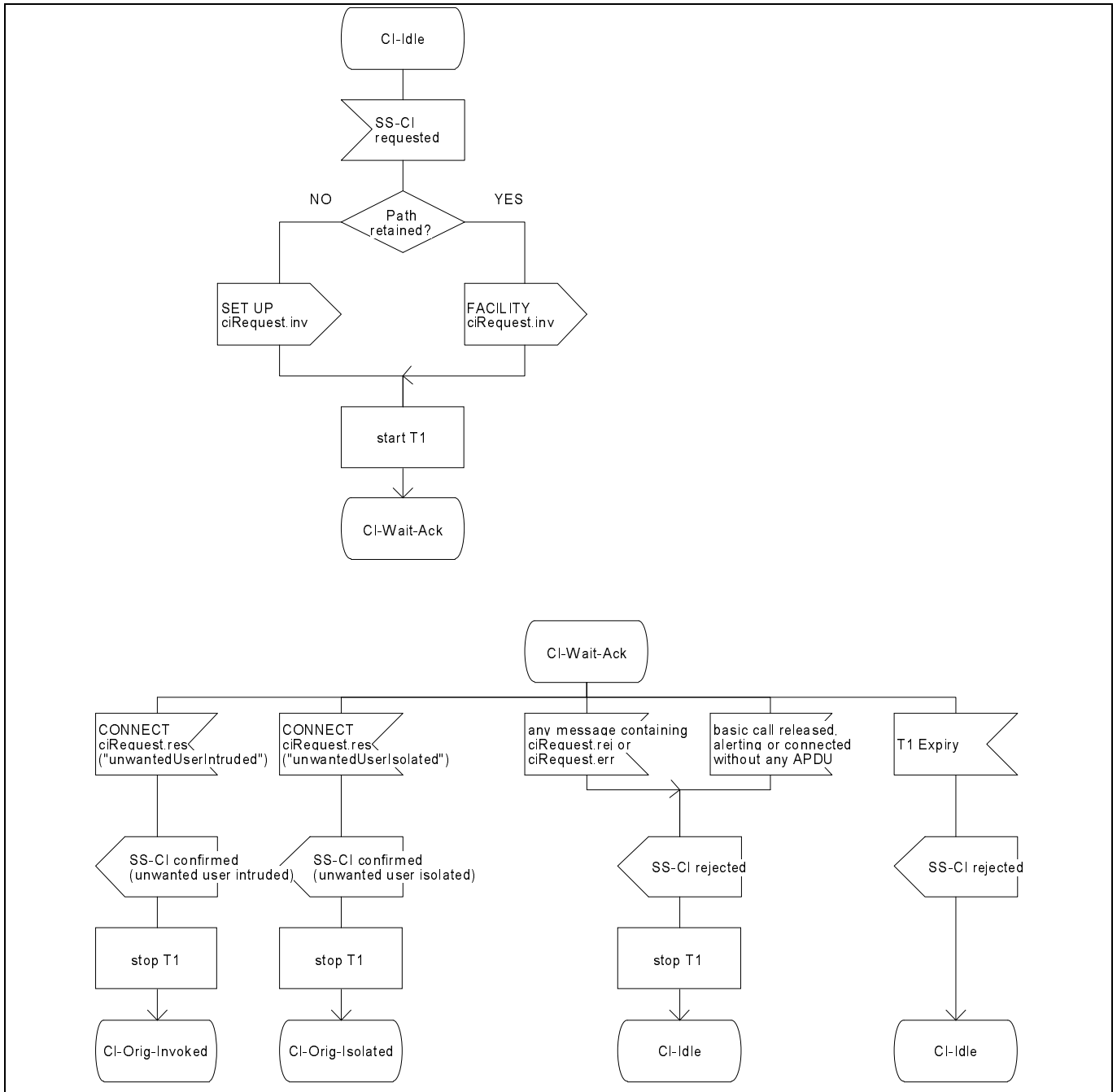
Figure D.1 (sheet 1 of 6) - Originating PTNX SDL
