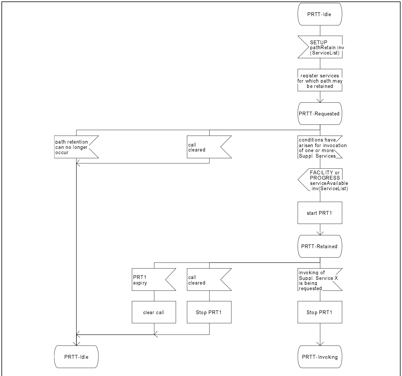
Figure A.2 (sheet 1 of 2) - SDL representation of Path Retention at the Terminating PTNX
