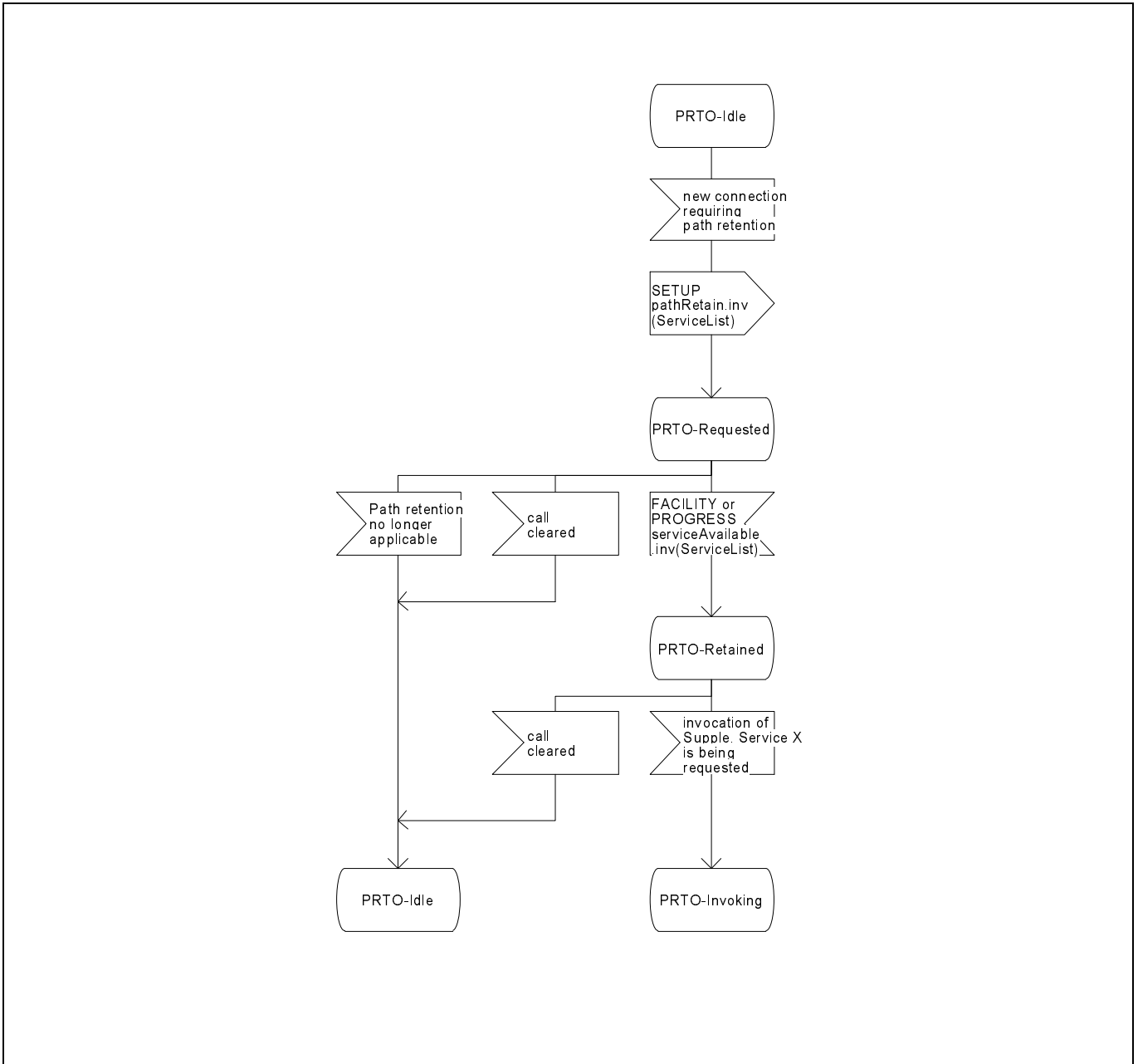
Figure A.1 (sheet 1 of 2) - SDL representation of Path Retention at the Originating PTNX
