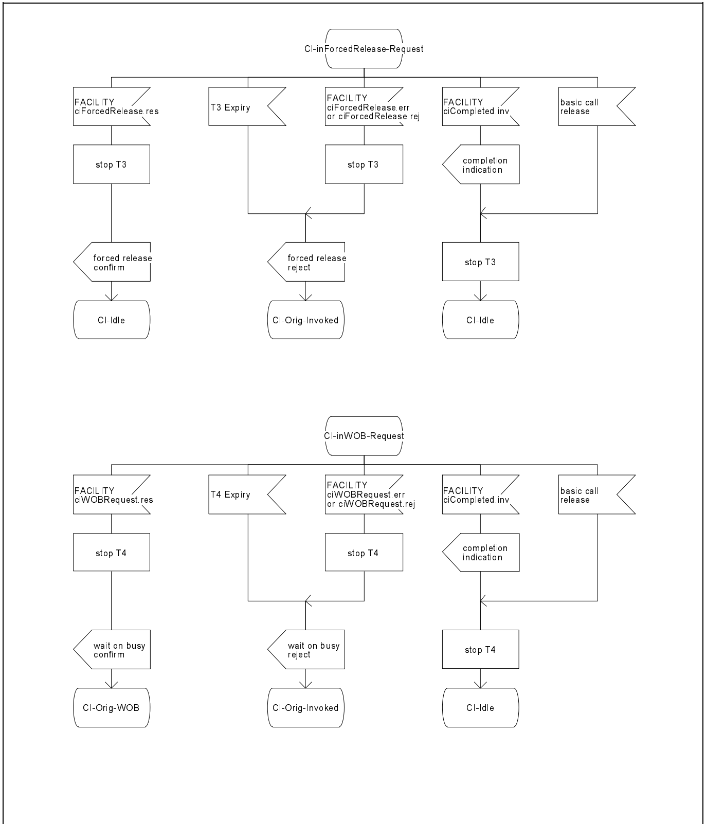
Figure D.1 (sheet 3 of 6) - Originating PTNX SDL
