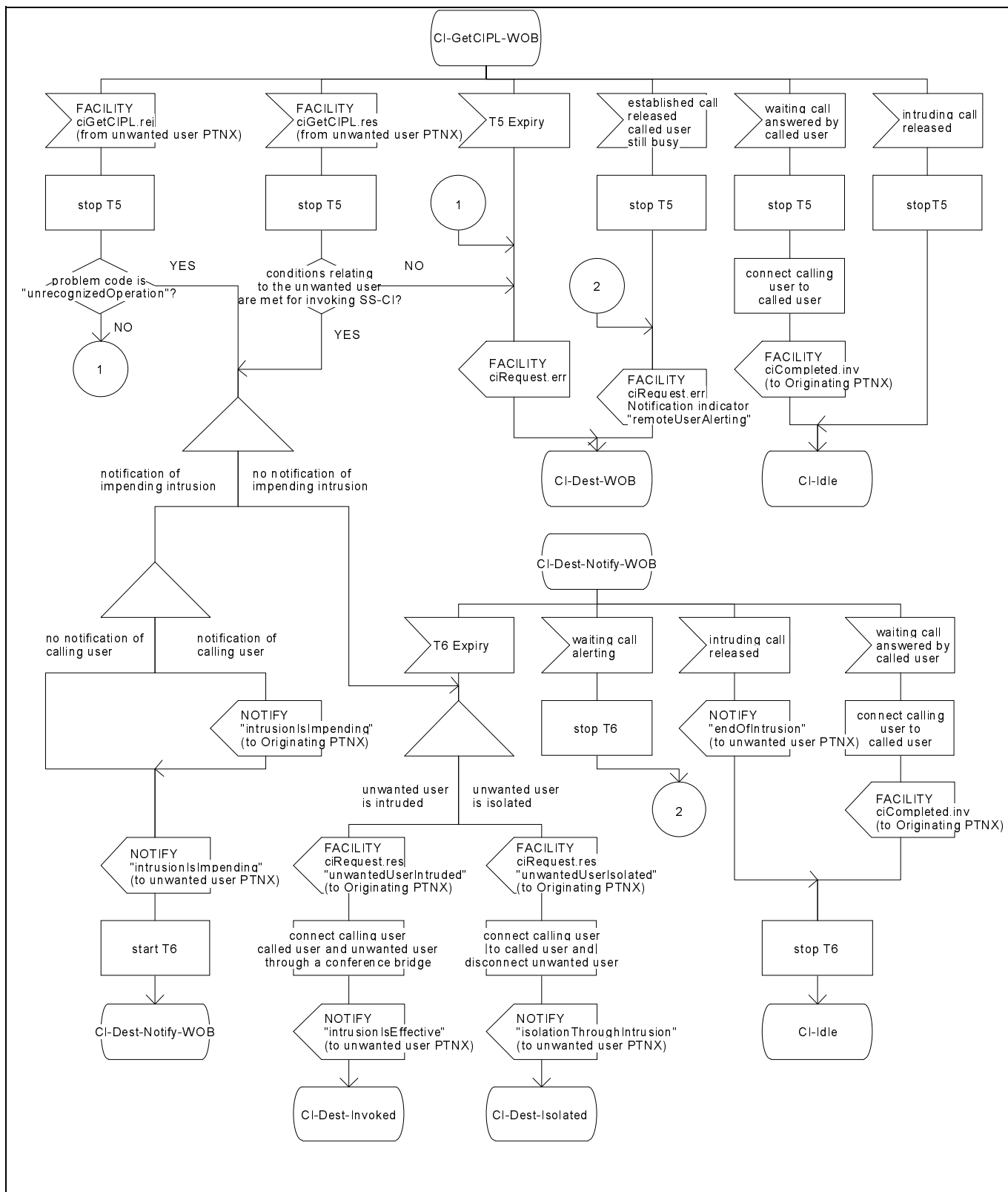
Figure D.2 (sheet 6 of 6) - Terminating PTNX SDL
