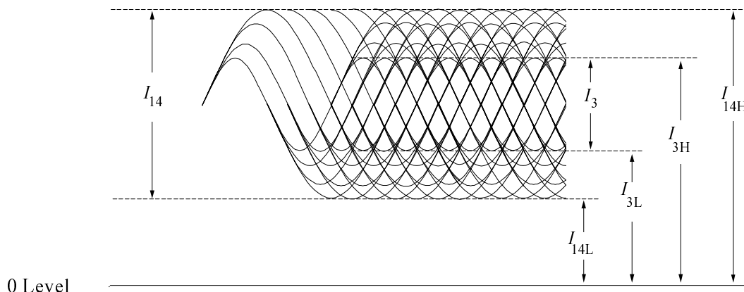
Figure 11 - Modulated amplitude
