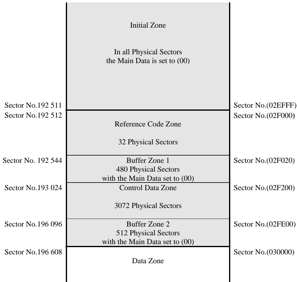
Figure 27 - Lead-in Zone
