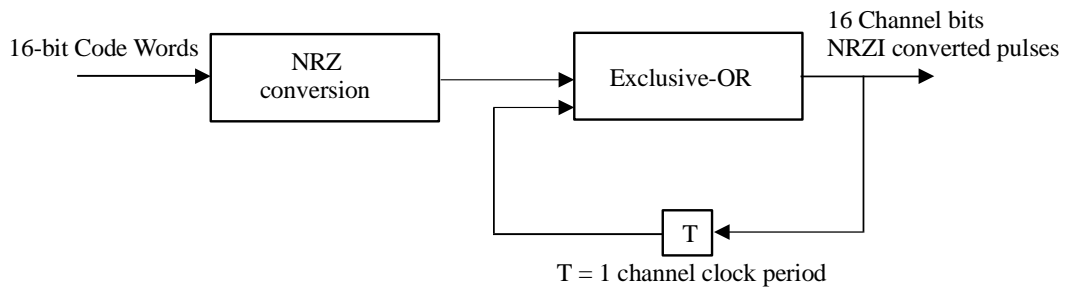
Figure 22 - NRZI conversion
