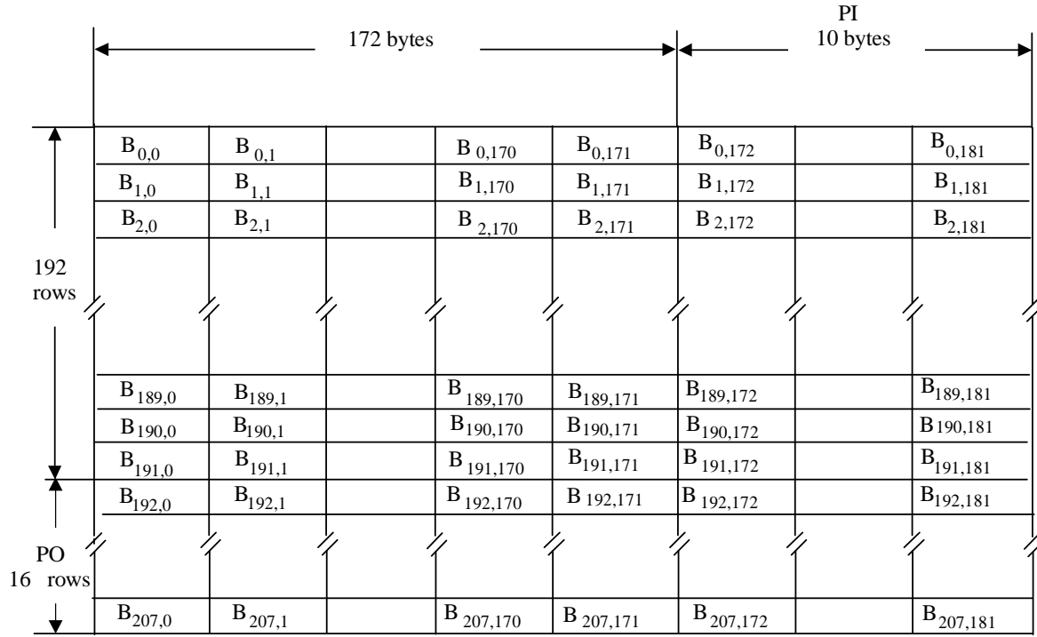
Figure 20 - ECC Block
