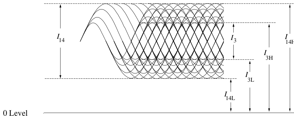
Figure 11 - Modulated amplitude
