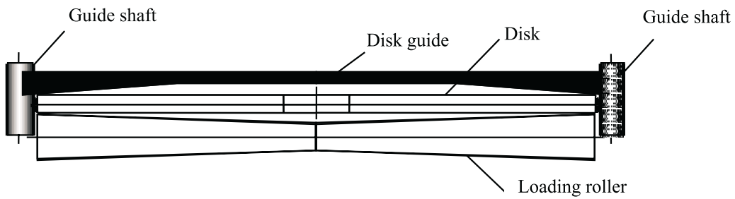
Figure N.5 - Slot-in mechanism
