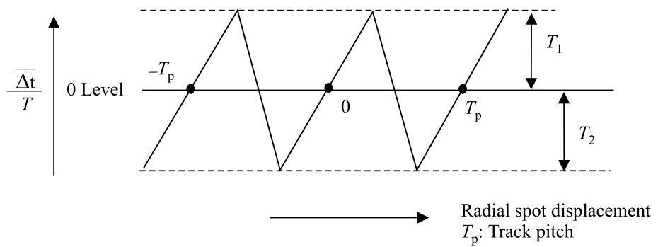
Figure 14 - Differential phase tracking error signal
