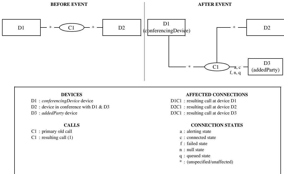
Figure 17-33 Conferenced Event—Case C: Join Call
