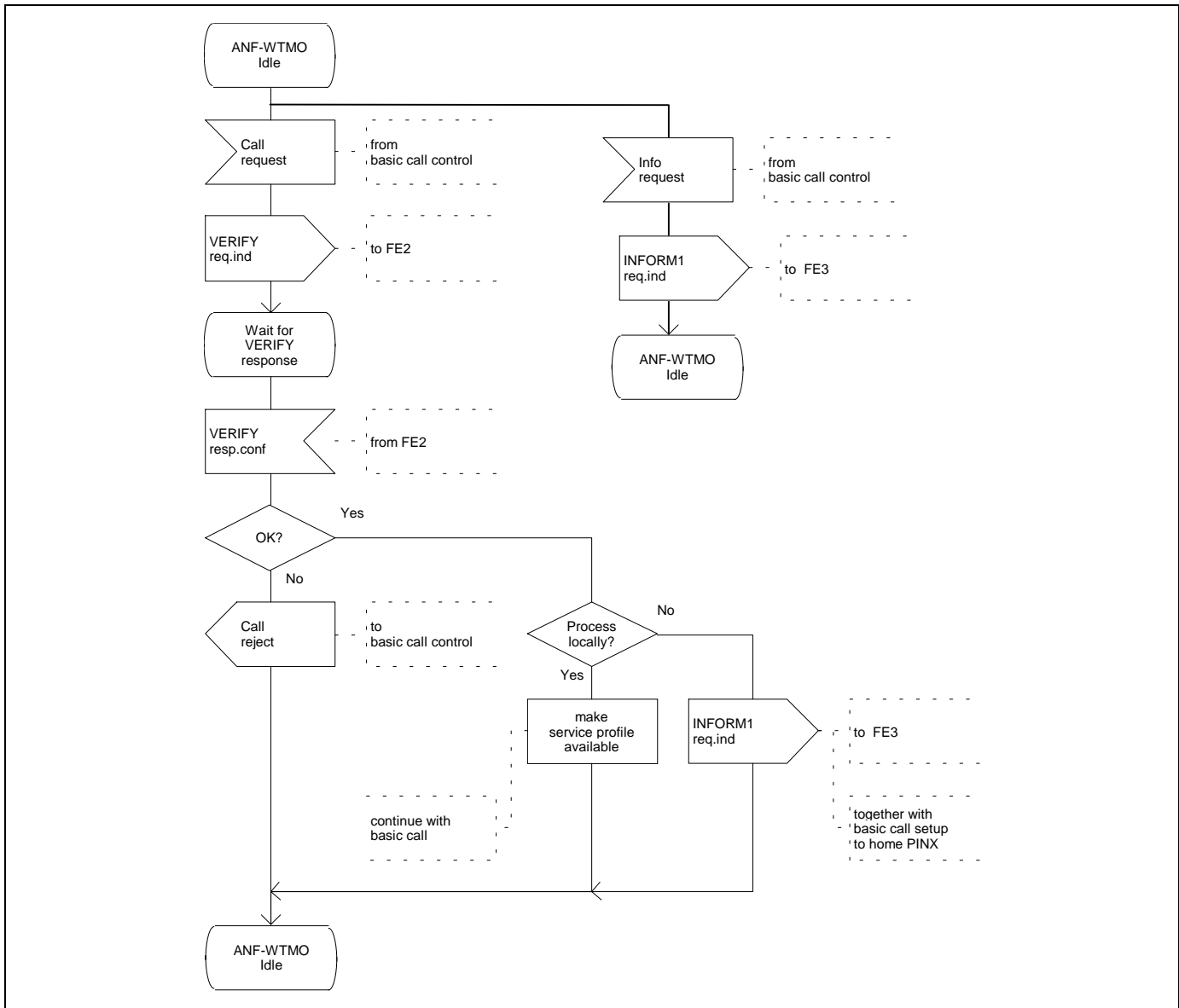
Figure 21 - ANF-WTMO, SDL for functional entity FE1
