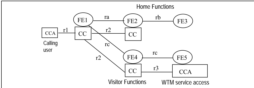
Figure 4 - Example relationship between model for ANF-WTMI and basic call
