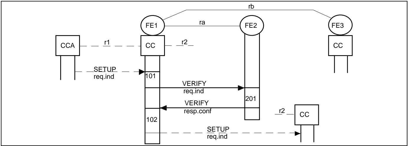
Figure 18 - Information flow sequence for successful WTMO operation: no redirection
