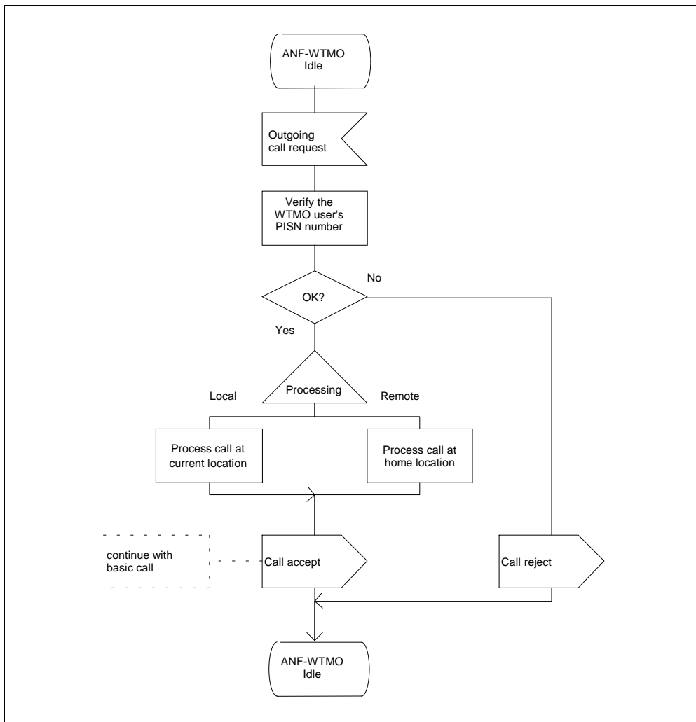
Figure 2 - ANF-WTMO, overall SDL
