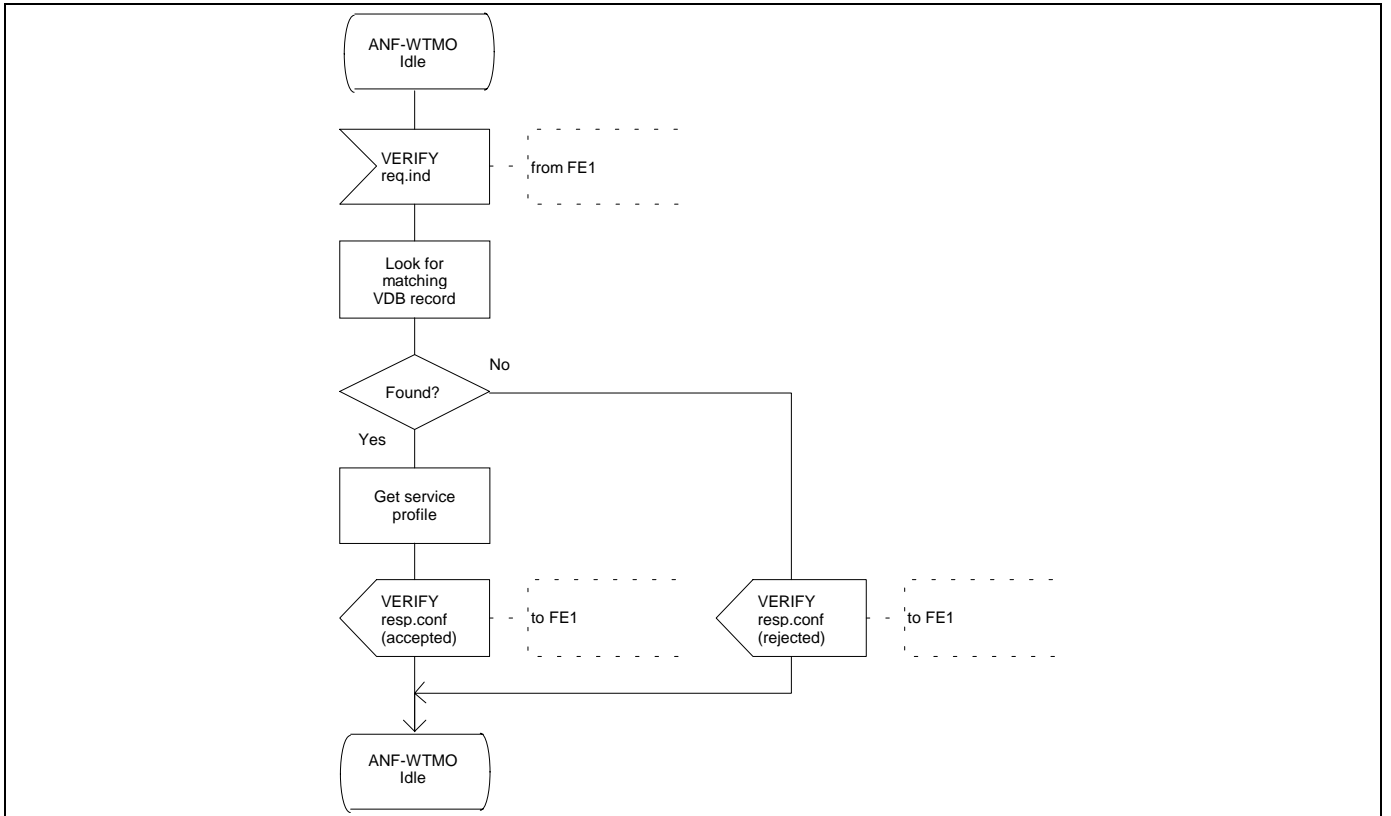
Figure 22 - ANF-WTMO, SDL for functional entity FE2
