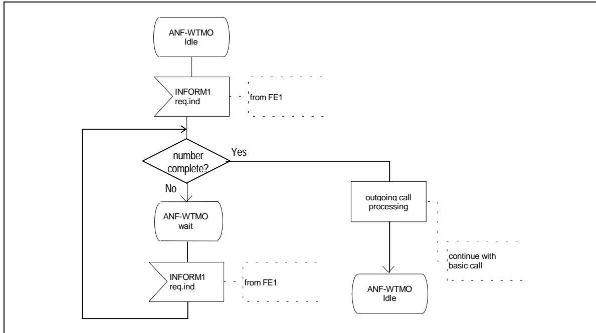
Figure 23 - ANF-WTMO, SDL for functional entity FE3
