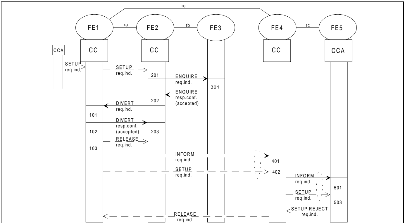
Figure 9 - Information flow sequence for unsuccessful WTMI operation: WTMI user not accessible
