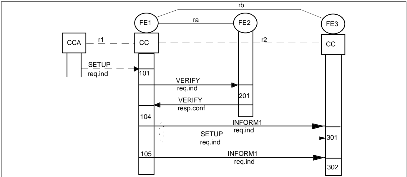
Figure 19 - Information flow sequence for successful WTMO operation: redirection to home location
