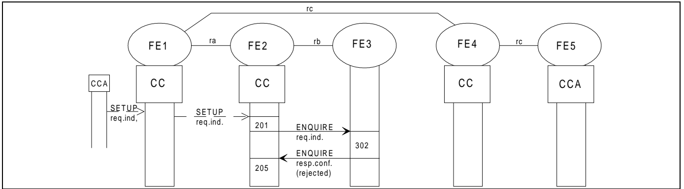
Figure 6 - Information flow sequence for unsuccessful WTMI operation: WTMI user (location) not known at home PINX or WTMI user deregistered
