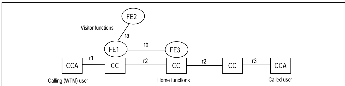
Figure 17 - Example relationship between model for ANF-WTMO and basic call
