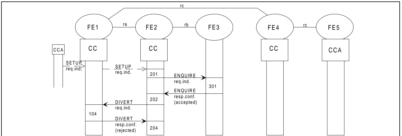
Figure 7 - Information flow sequence for unsuccessful WTMI operation: rejection of diversion
