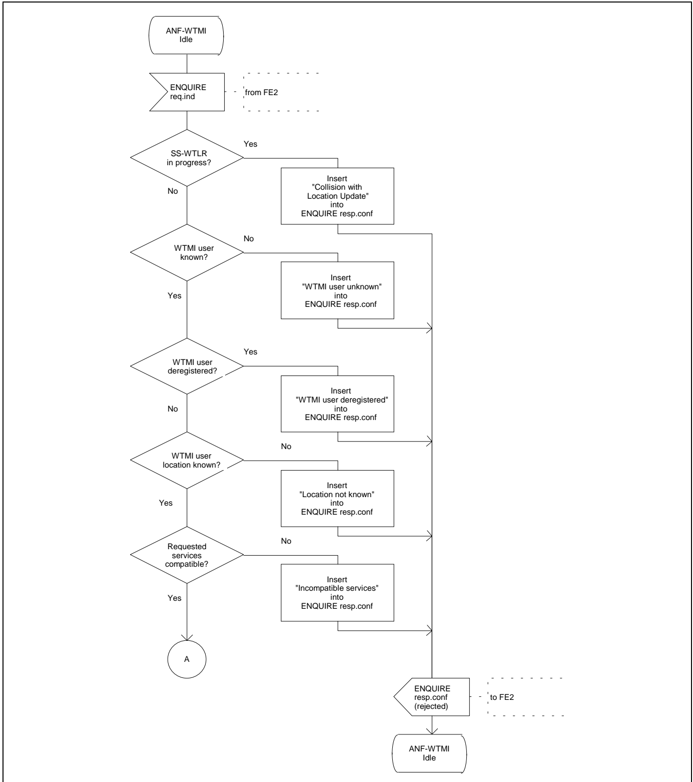
Figure 12 - ANF-WTMI, SDL for functional entity FE3 (page 1 of 2)
