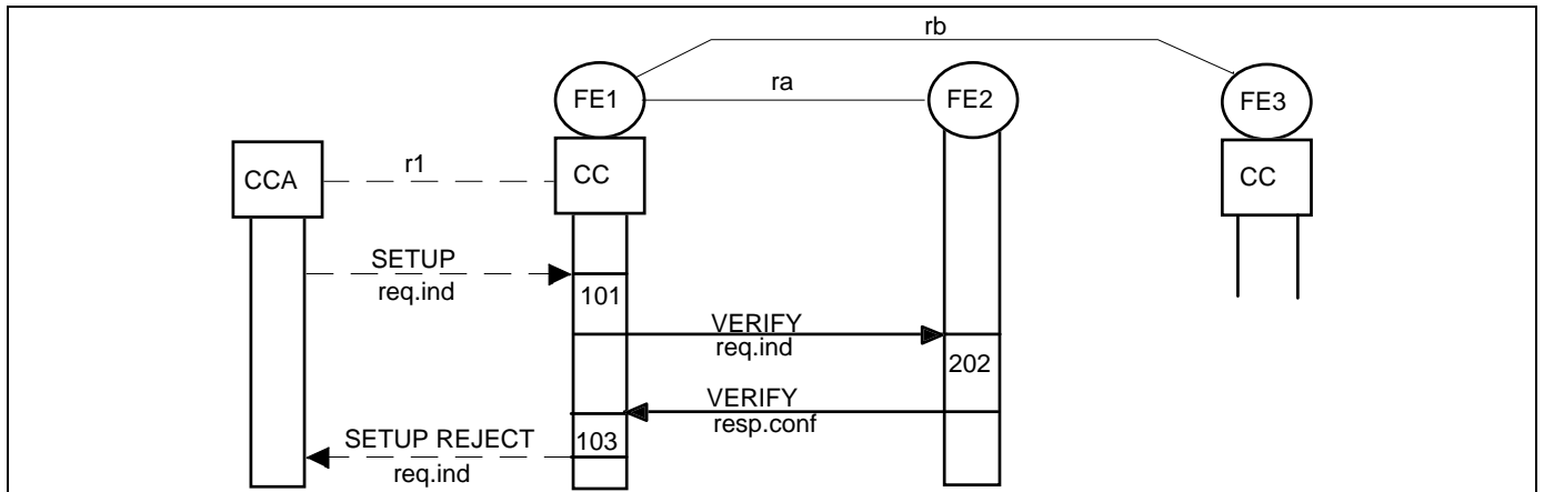
Figure 20 - Information flow sequence for unsuccessful WTMO operation: no matching VDB record found
