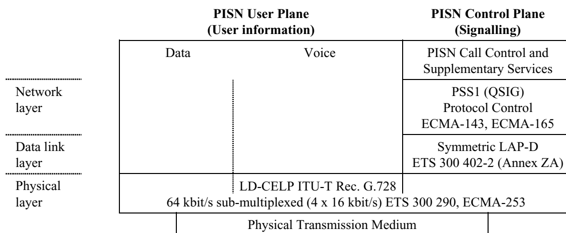
Figure 2 - Protocol stack
