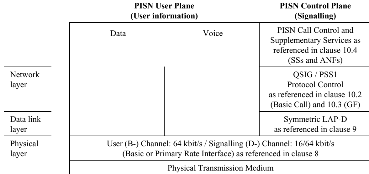
Figure 2 - Protocol Stack
