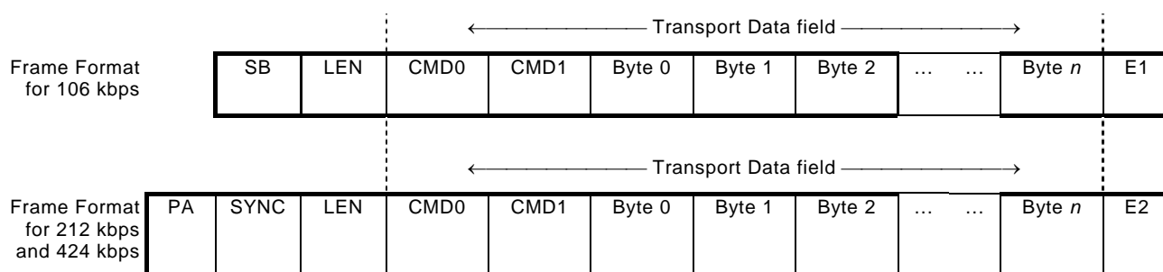
Figure 23 — Transport Frame format Definition
