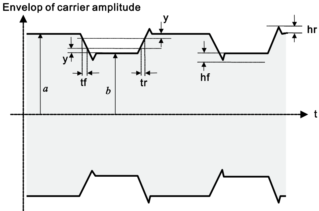
Figure 2 — Modulated Waveform
