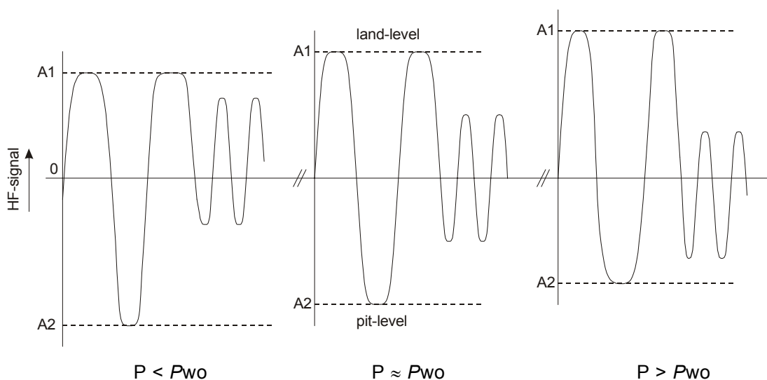
Figure H.2 - AC-coupled HF signals recorded with different writing powers
