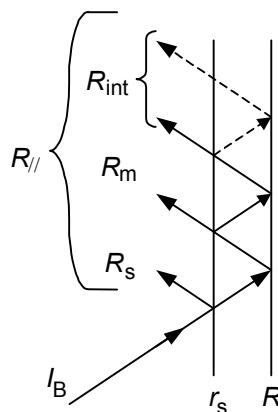
Figure B.1 - Reflectivity calibration
