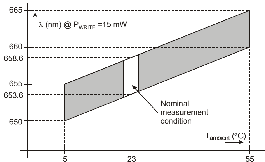
Figure J.1 - Wavelength/Temperature diagram indicating the disk operating conditions
