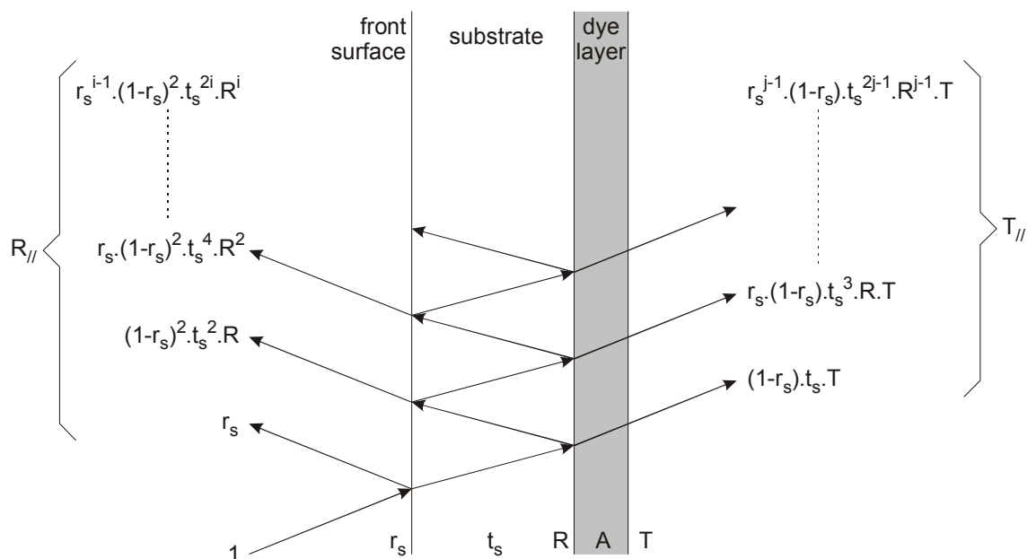
Figure J.2 – Definitions of reflectivity, transmission and absorption
