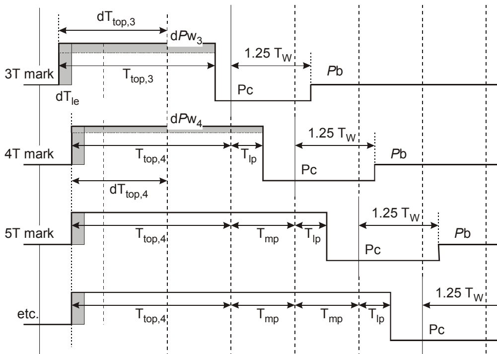
Figure F.4 - Examples of a "blocked" waveform
