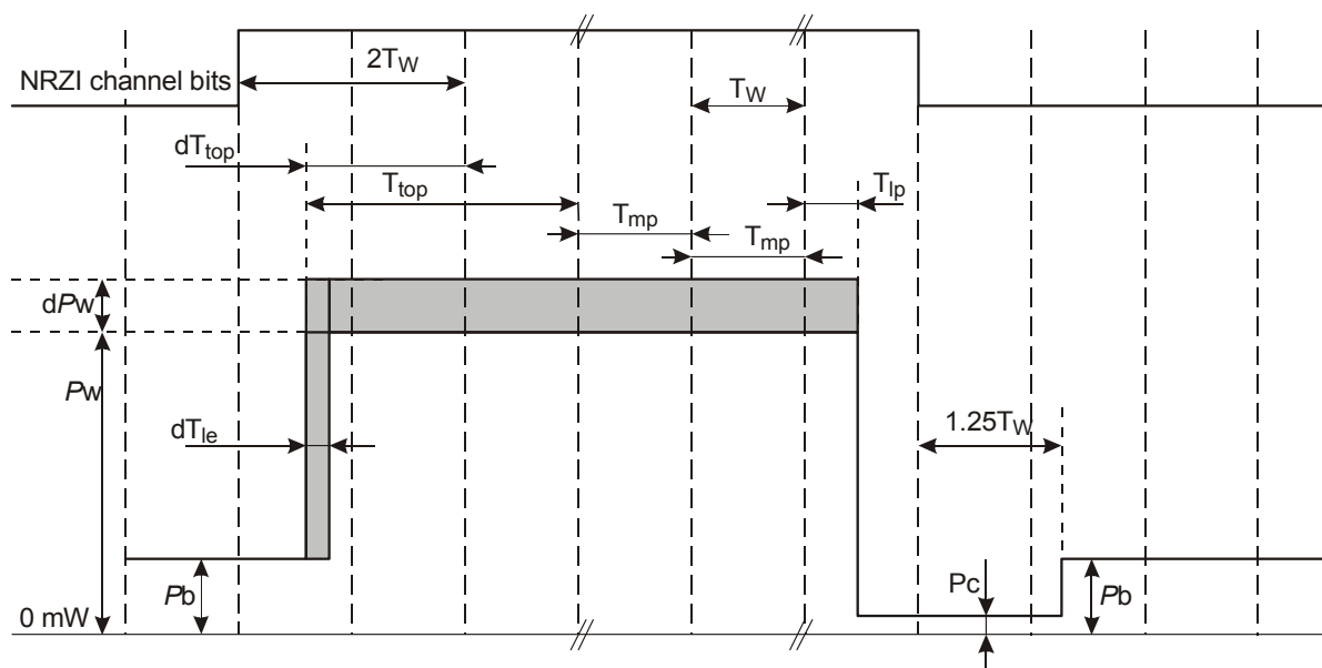
Figure F.3 – General blocked waveform
