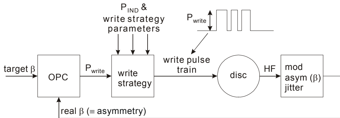
Figure H.1 - Schematical diagram of OPC procedure
