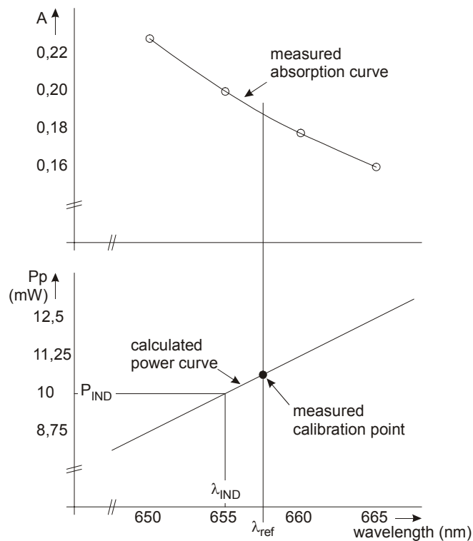
Figure J.3 – Example of absorption and power versus wavelength
