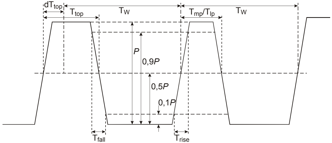
Figure F.5 - Rise Times and Fall Times
