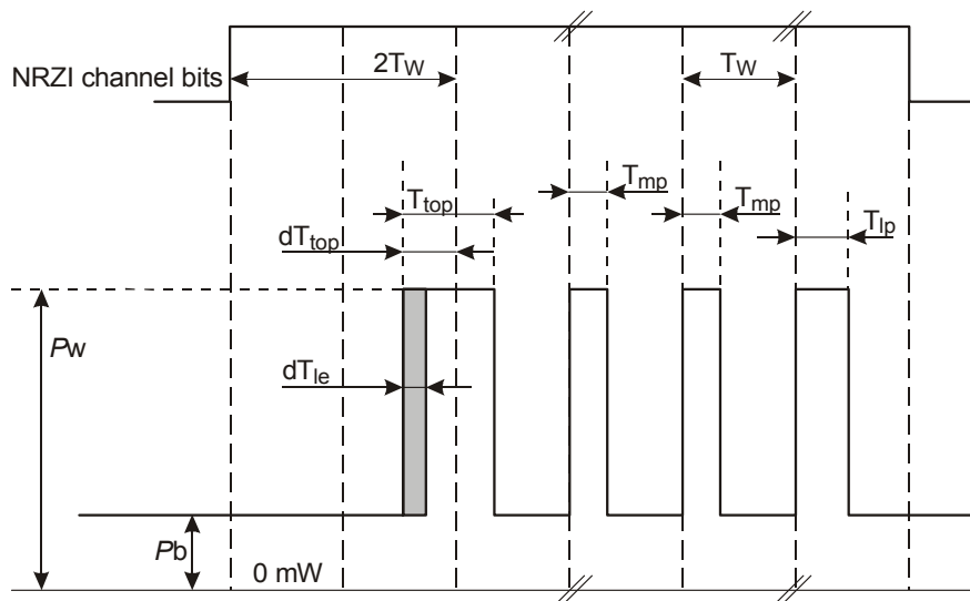
Figure F.1 - Write pulse waveform
