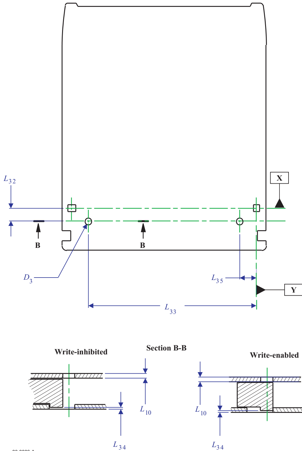
Figure 7 – Write-inhibit holes
