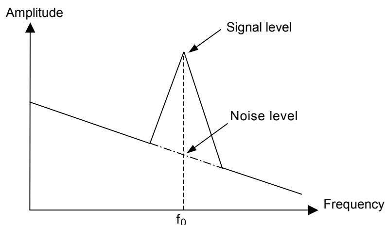
Figure 30 – Amplitude versus frequency for the Phase Change signal
