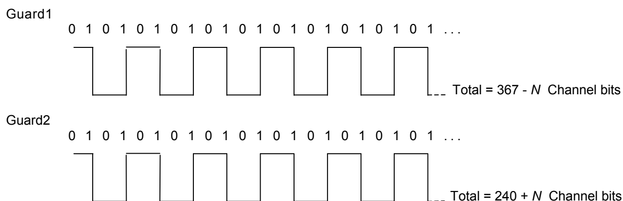
Figure 24 – Guard field patterns
