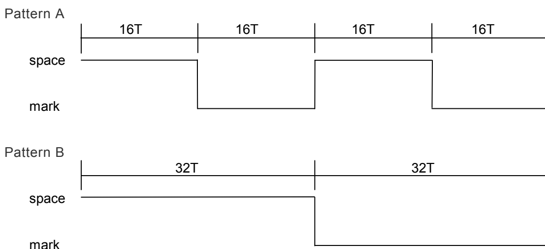
Figure 23 – Quadrature Wobble Mark field patterns
