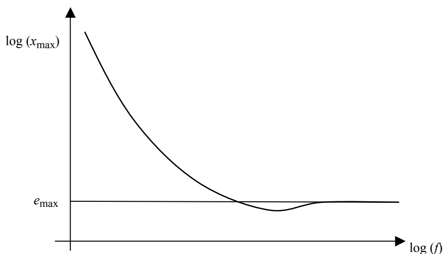
Figure V.1 – Maximum allowed amplitude of a single, sinusoidal track deviation
