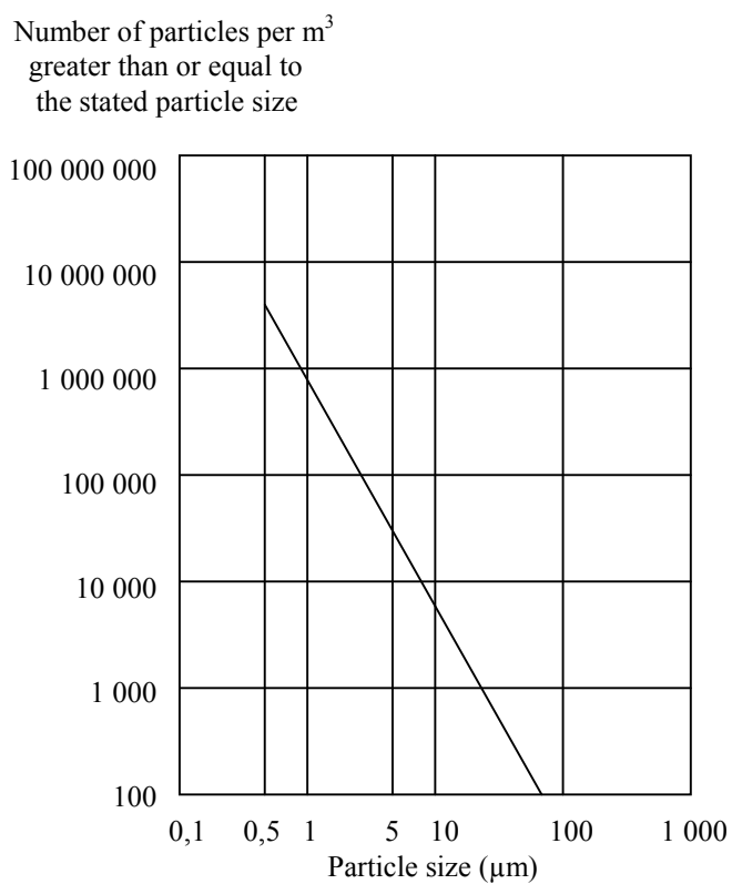
Figure A.1 – Particle size distribution curve
