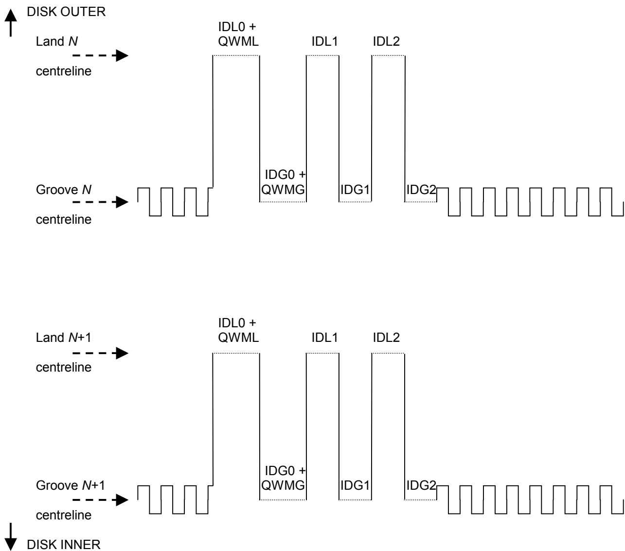
Figure 16 – Preformatted Header and wobble groove displacements
