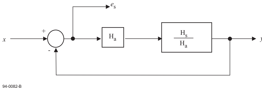
Figure V.3 – Implementation of a Reference Servo by changing the transfer function of the actual servo
