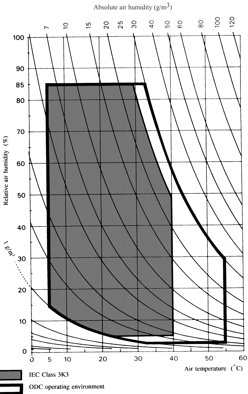
Figure T.1 – Climatogram of IEC Class 3K3 and the ODC operating environment
