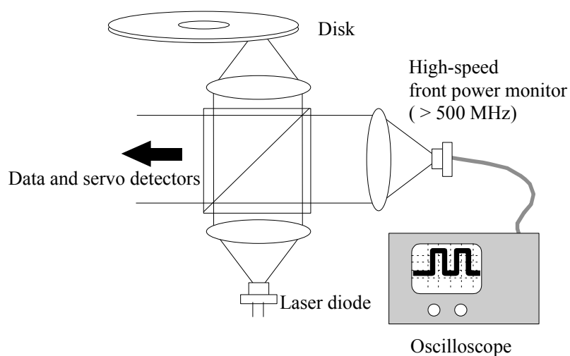
Figure CC.2 – Measurement of pulse power and pulse width
