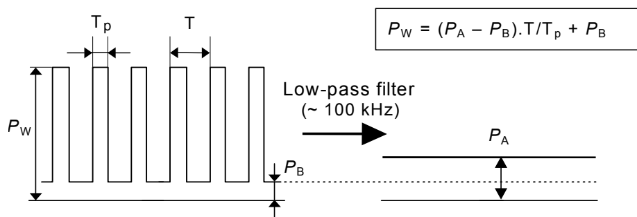
Figure CC.3b – Determination of pulse power level P_W from average power level P_A
