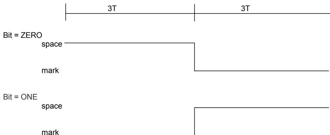
Figure 27 – STOB bit patterns
