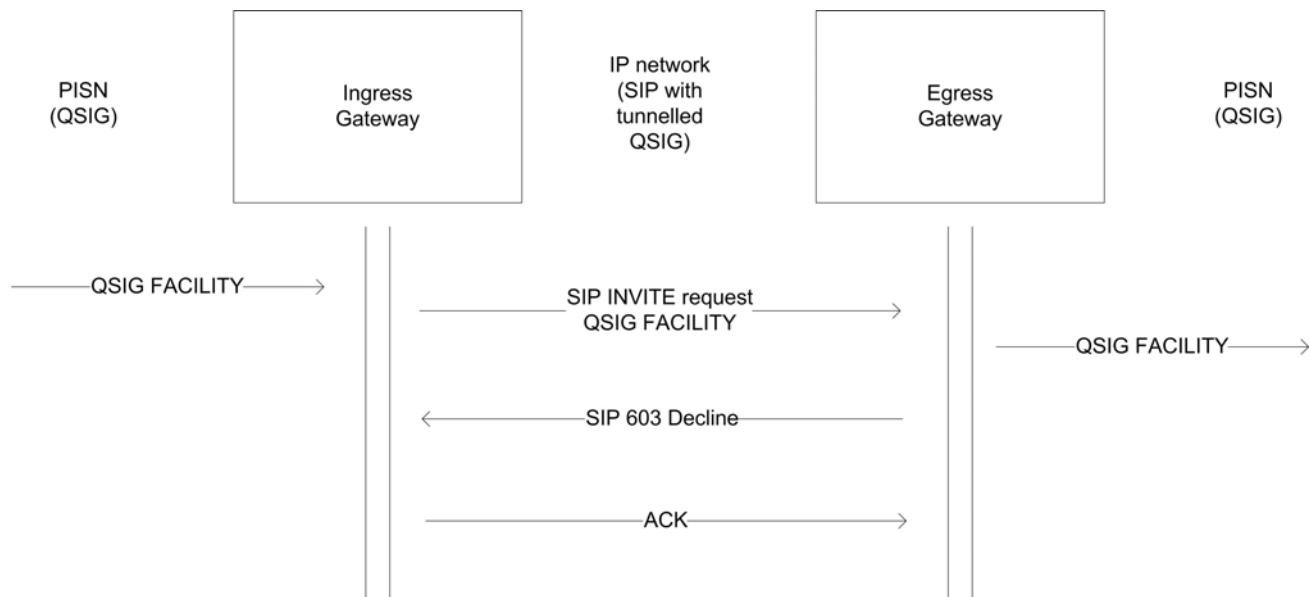
Figure 4 – QSIG call independent connectionless signalling
