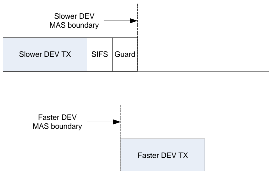
Figure 105 - Guard Time
