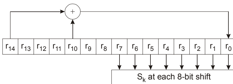
Figure 12 - Feedback shift register
