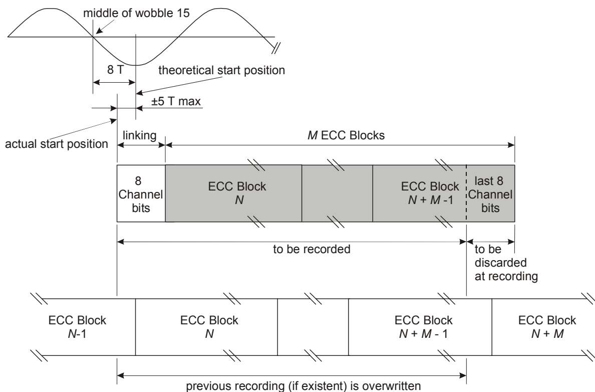
Figure 17 - Recording Unit
