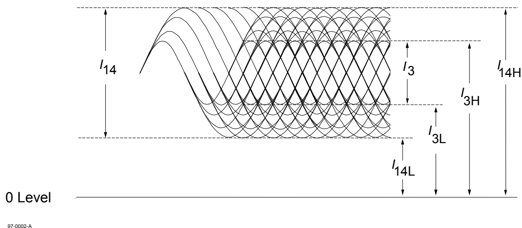
Figure 26 — Signals from spaces and marks in Read channel 1
