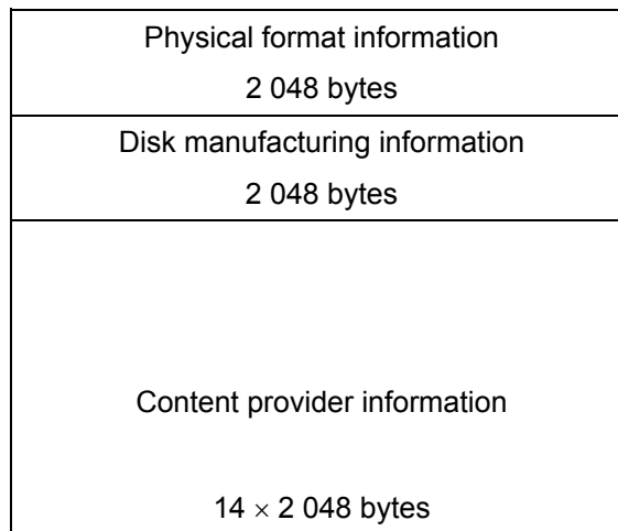
Figure 23 — Structure of a Control Data Block
