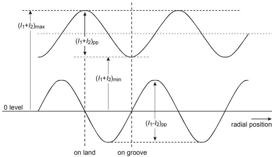
Figure 25 — Signals from grooves in the Read Channels when crossing the tracks
