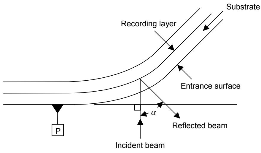
Figure 9 — Angular deviation
