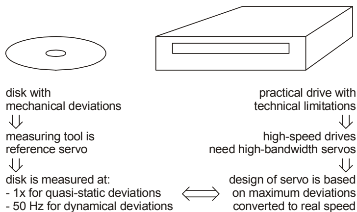
Figure K.1 — Illustration of disk measurement and drive design
