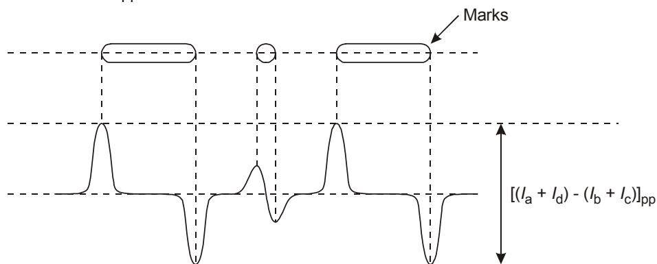
Figure 29 — Tangential push-pull signal
