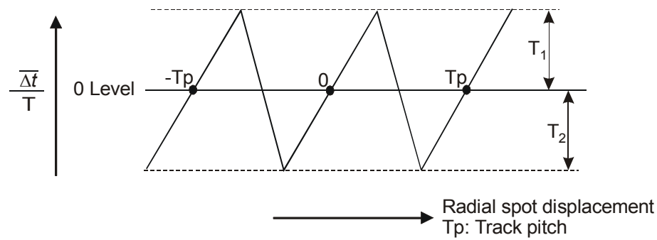
Figure 28 — Differential phase tracking error signal
