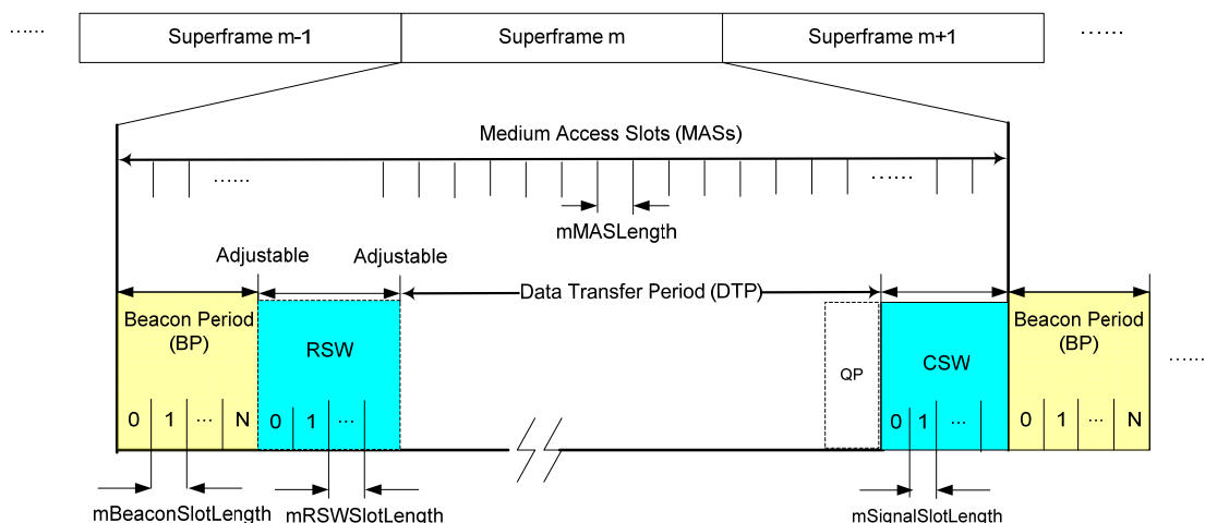
Figure 14 — Data Period
