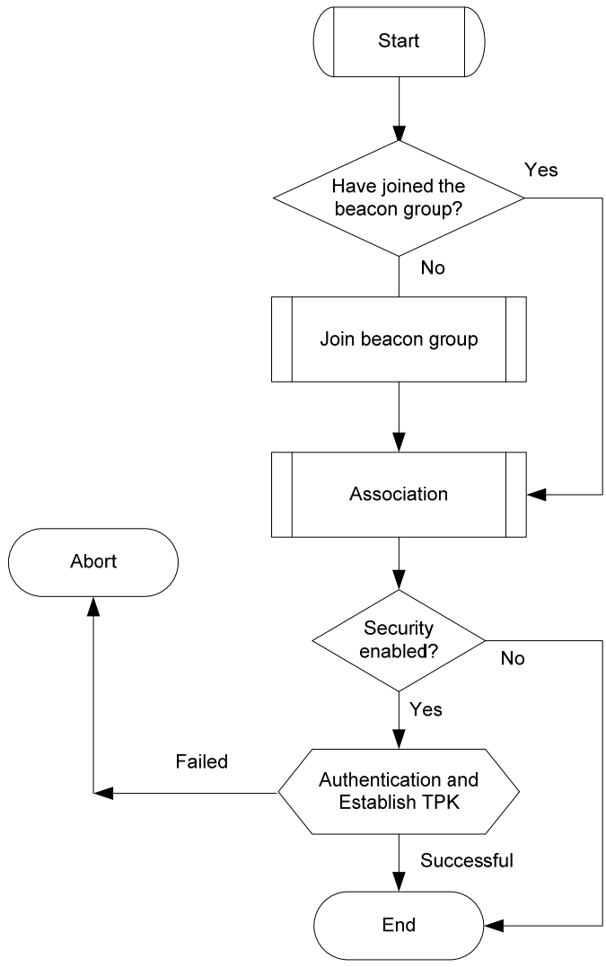
Figure 25 — Pairing Procedure
