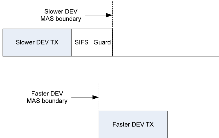
Figure 11 — Guard Time
