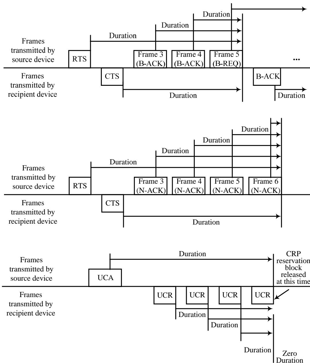
Figure 8 — Duration examples
