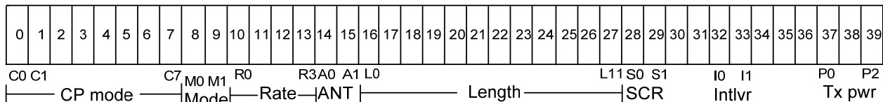
Figure 33 — PHY header format
