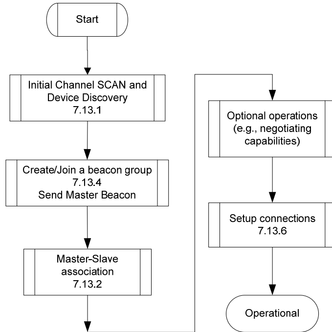
Figure 21 — Network Entry Procedure for A Master Device
