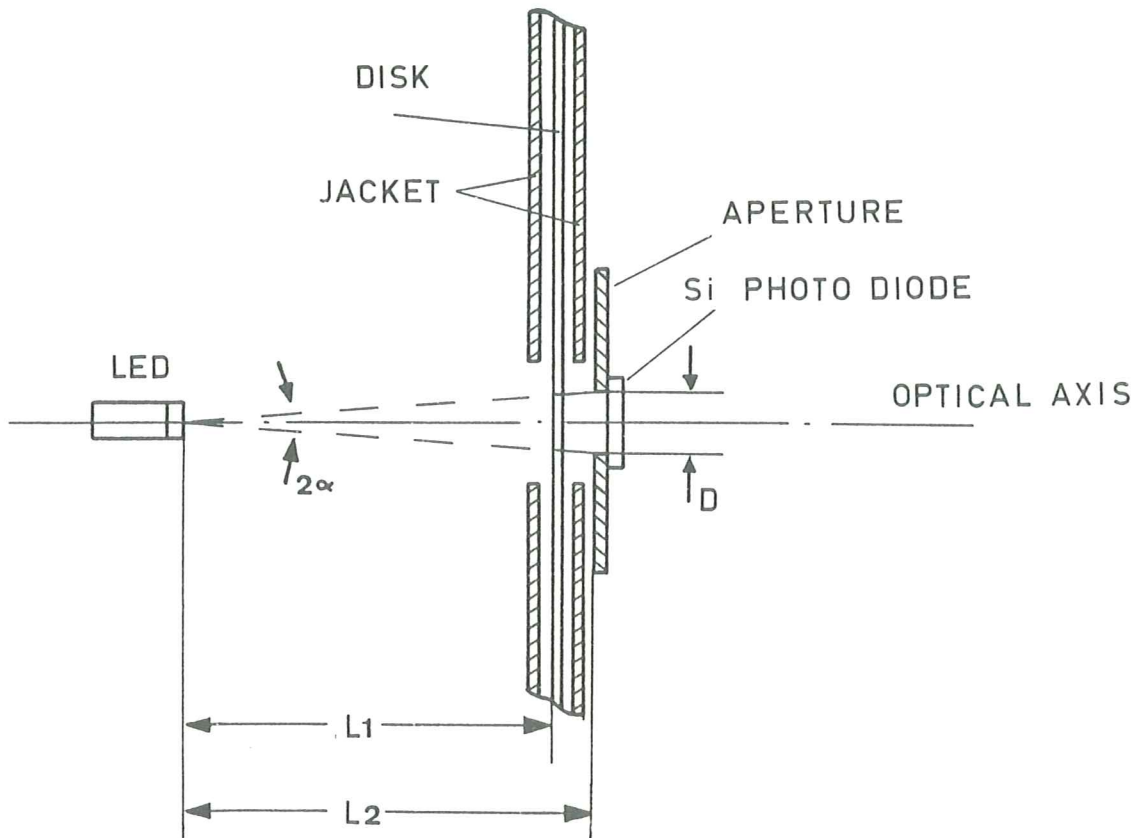
FIG. 1 MEASURING DEVICE
