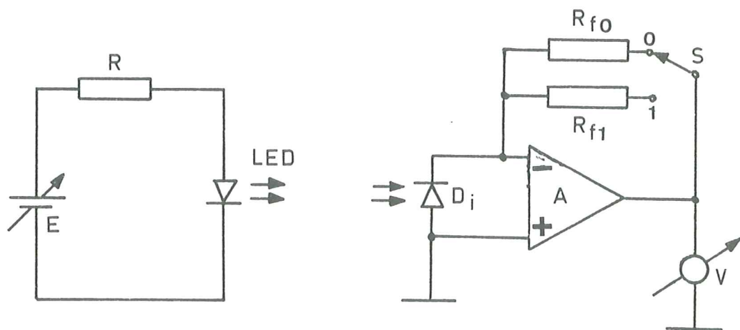
FIG. 2 ELECTRONIC CIRCUITRY
