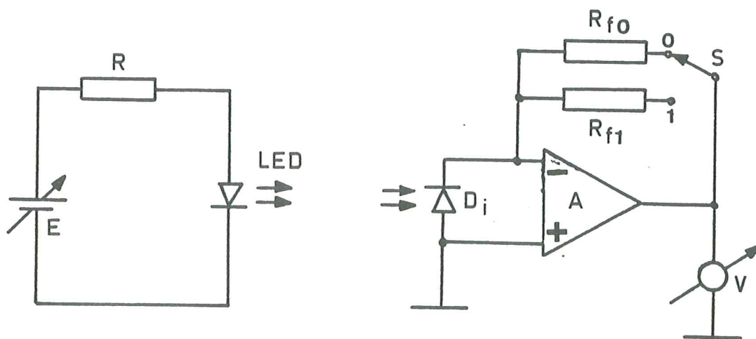
FIG. 2B ELECTRONIC CIRCUITRY
