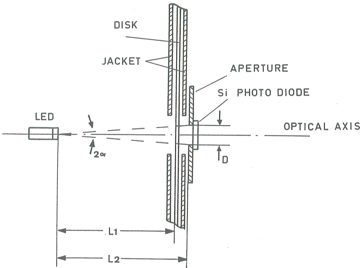
FIG. 1B MEASURING DEVICE
